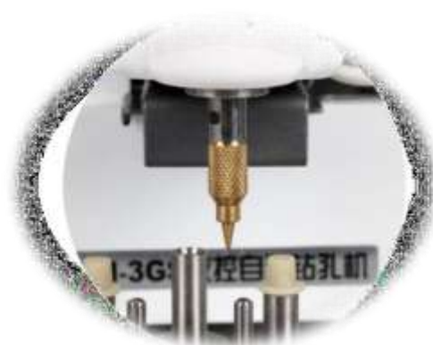
Drill specifications: \varnothing 1.0 , \varnothing 1.2 , \varnothing 1.42 , \varnothing 1.5 , \varnothing 1.6 , \varnothing 1.7 , \varnothing 2.0 , milling cutter 1.1, measuring tip.
